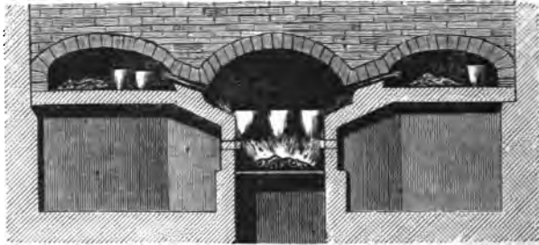
Fig. 10.—Glass Furnace.
