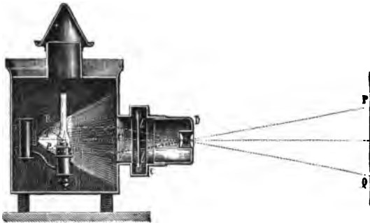
Fig. 57.—Magic Lantern.
