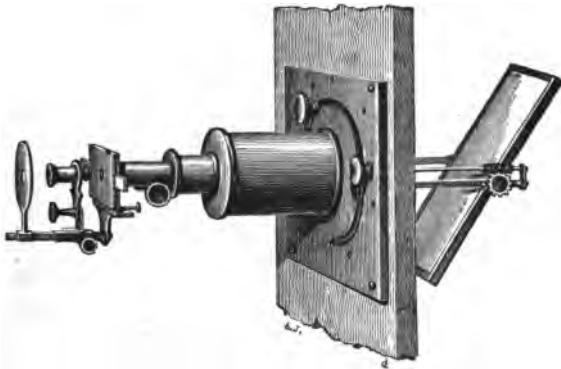
Fig. 58.—Solar Microscope.
