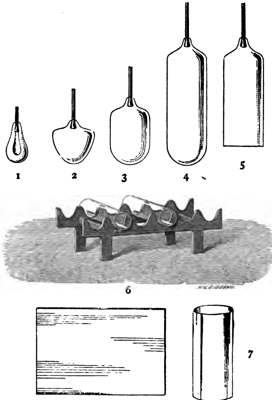
Fig. 12.—Blowing of Sheet Glass.
