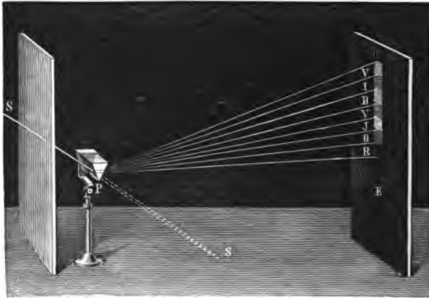
V Violet. I Indigo. B Blue. V Green. J Yellow. O Orange. R Red.
