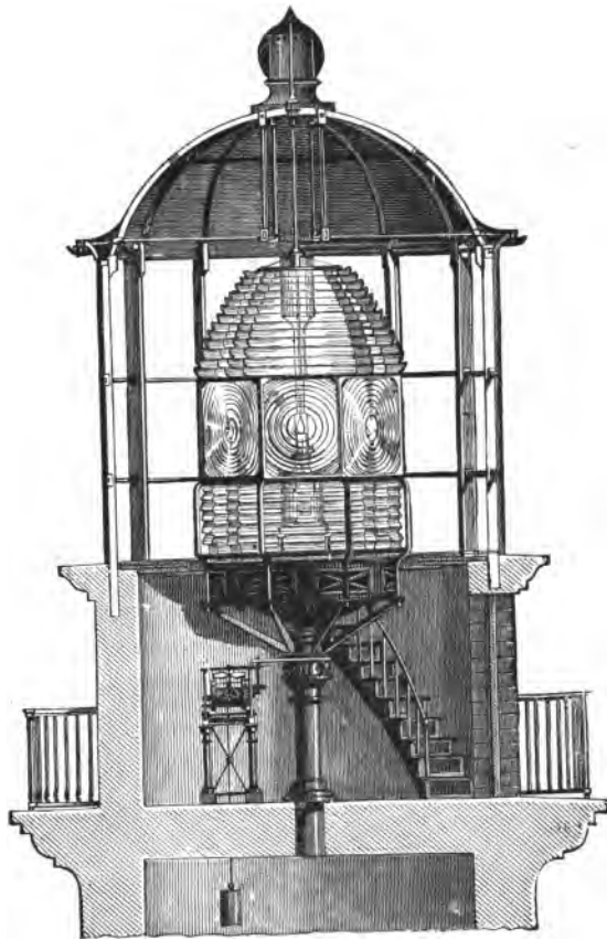
Fig 67.—Lighthouse Lantern
