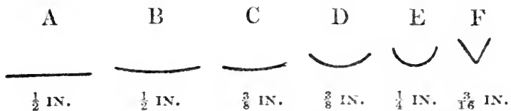
FIG. 5.—SET OF SIX CARVING TOOLS. A, CHISEL; B AND C, FLAT GOUGES; D AND E, BENT GOUGES; F, V-TOOL
