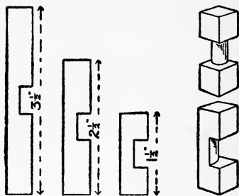
Fig. 409. Fig. 410. Fig. 411. Fig. 412. The Three Cross Pieces. Key Piece,
