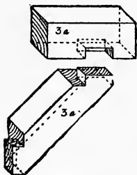
Fig. 32.—Oblique Halving, with Shoulder.
