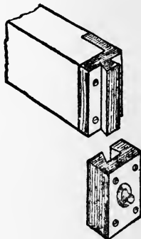
Fig. 373.—Bed Joint.
