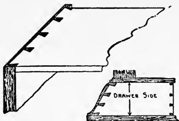
Fig. 303.—Lap-Dovetailing. Fig. 304.—Jewel Drawer Side.
