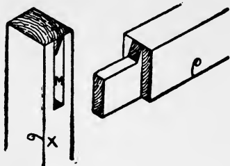
Fig. 184.—The Joint Separated.
