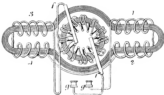
Circuit of simple electric motor.
