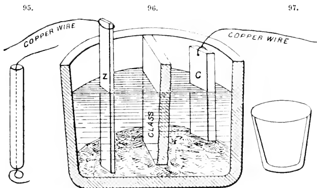
Selby's battery.
