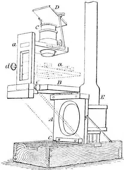
Portable lantern.
