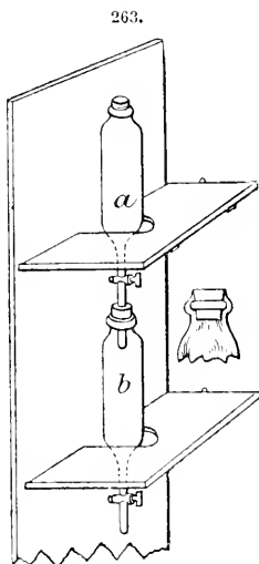
Repercolator.
