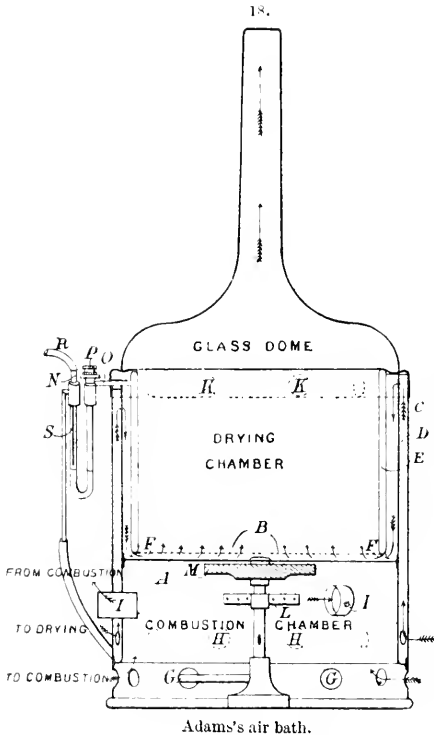
Adams's air bath.
