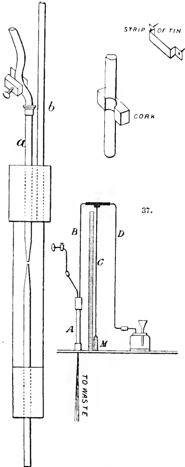
Vacuum pump for hastening filtration.
