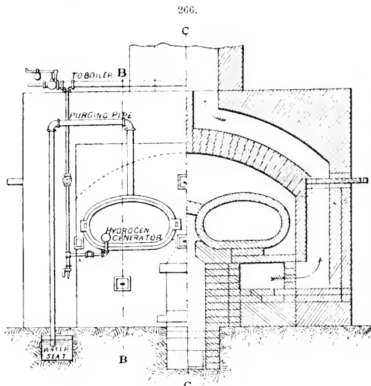
Gesner's rust-proofing furnace.
