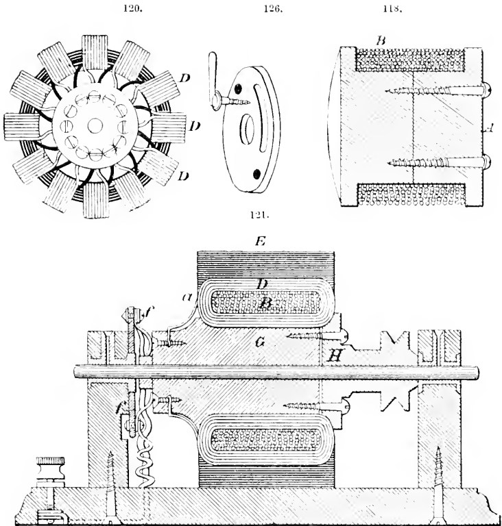
Fig. 118, armature core; fig. 121, transverse section; fig. 120, end view of armature showing commutator; fig. 126, brush-holding disc.
