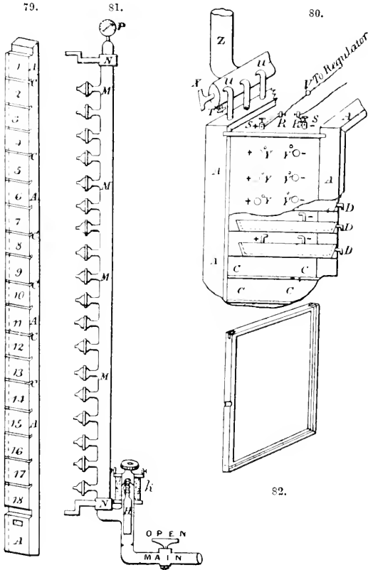
Trechby's battery.
