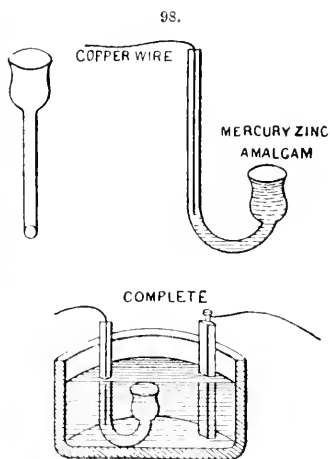
Selby's battery.
