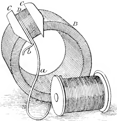
Winding the armature.
