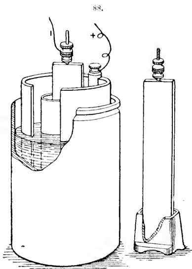
Radiguet's 2-liquid battery.
