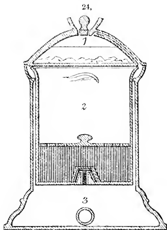
Paulson's filter.
