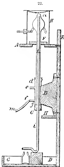
Mercury still.
