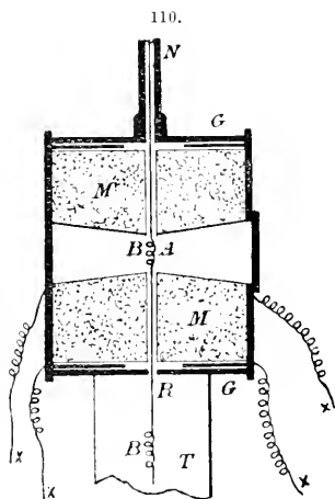
Section of Galvanometer.
