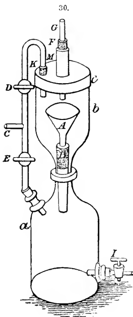
Precipitate filter.
