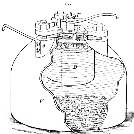
Lalande-Chaperon battery.
