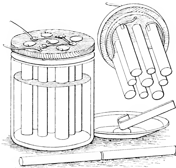
Single fluid battery.
