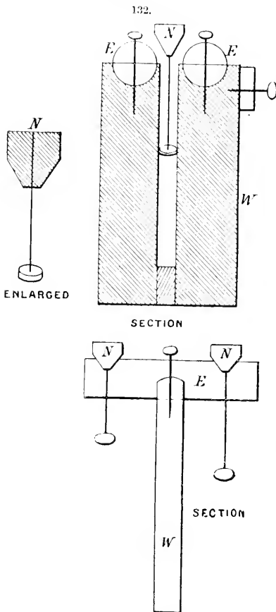
Microphone transmitter.
