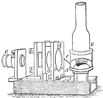
Portable lantern.
