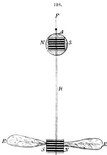
Galvanometer needle.
