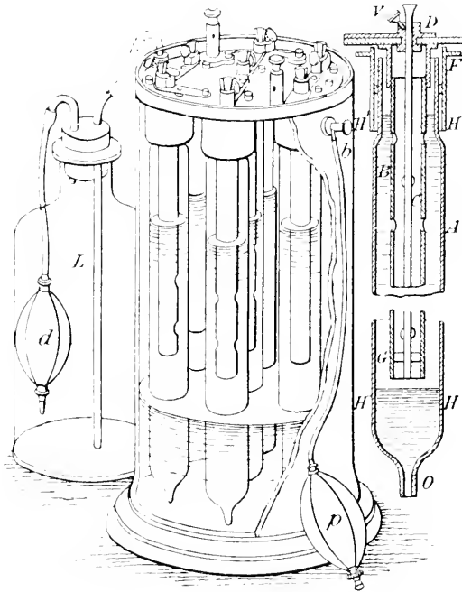
Pneumatic battery for electric lighting.
