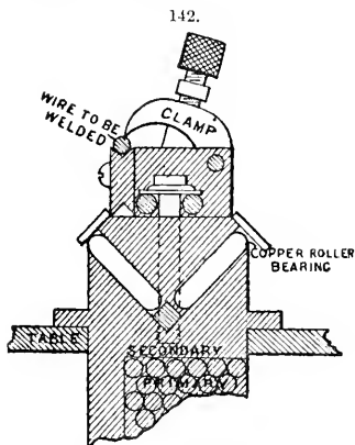
Arrangement of Clamps.
