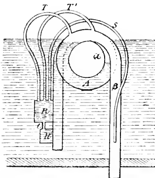
Siphon for intermittent discharge.
