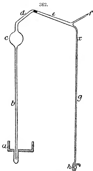
Filling barometer tubes.
