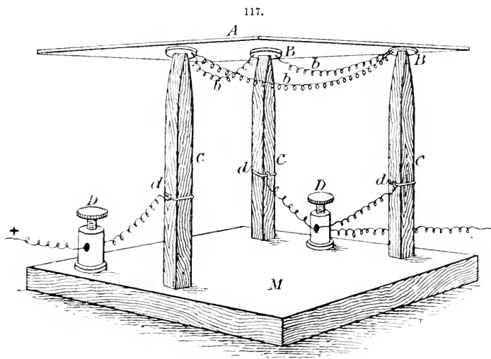
Easily constructed microphone.
