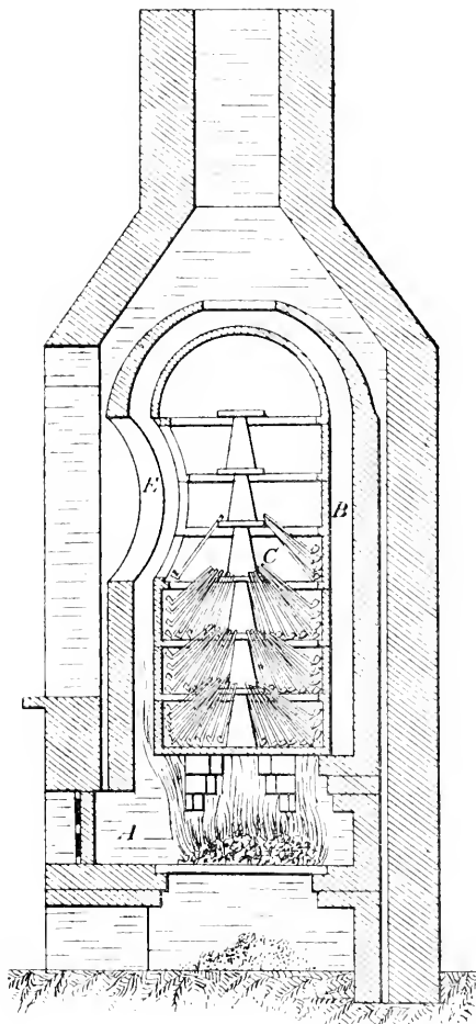
Pipe-makers' oven.
