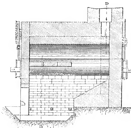
Gesner's rust-proofing furnace.
