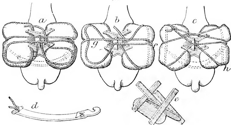
Diamond hitch.
