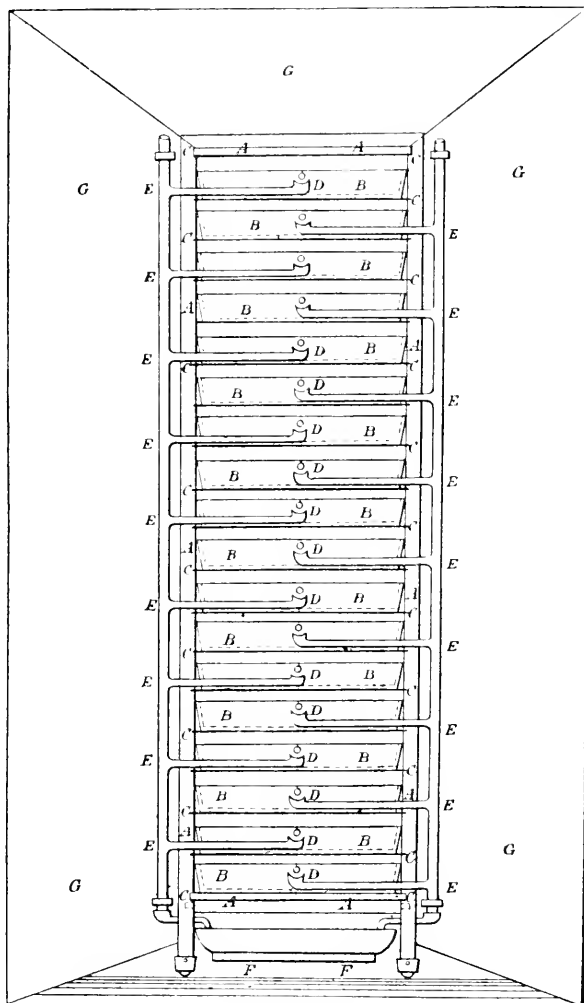
Treeby's battery.
