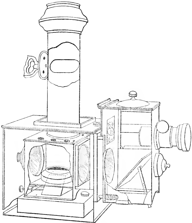
Pentaplane lamp.
