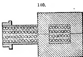
Transformers.
