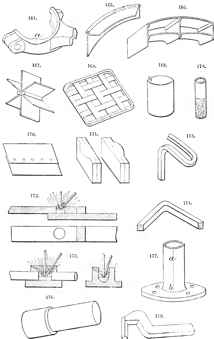
Electric welding.
