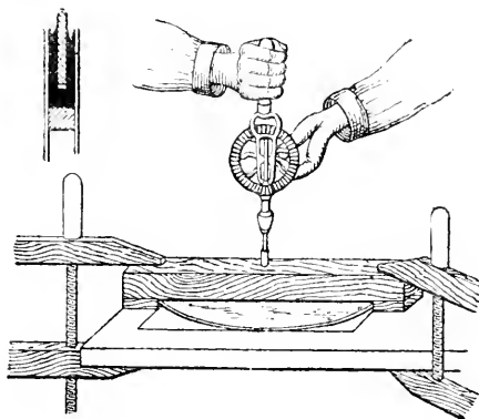
Drilling glass.
