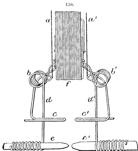
Regulator.
