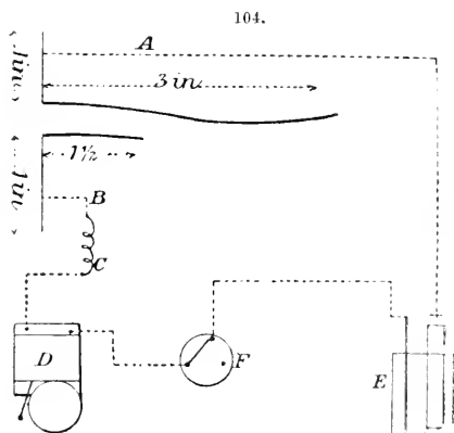
Bell to ring by opening door.
