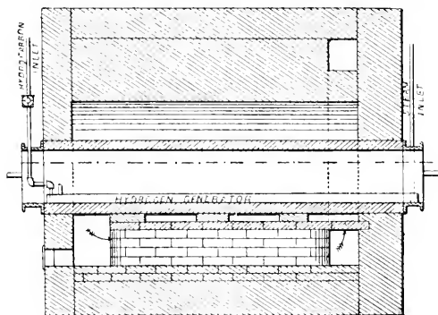
Gesner's rust-proofing furnace.
