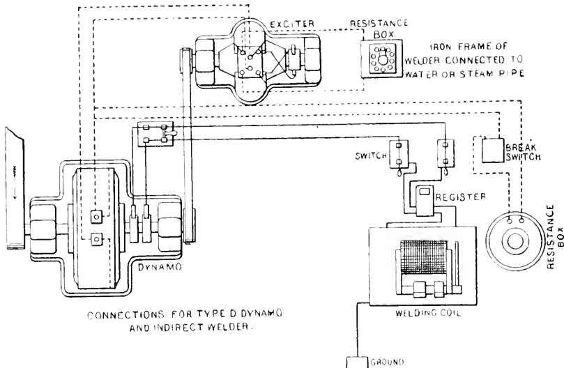
Electric welding apparatus.
