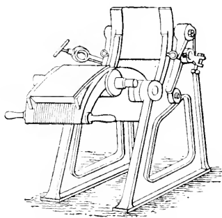
Casting-box for curved plates.
