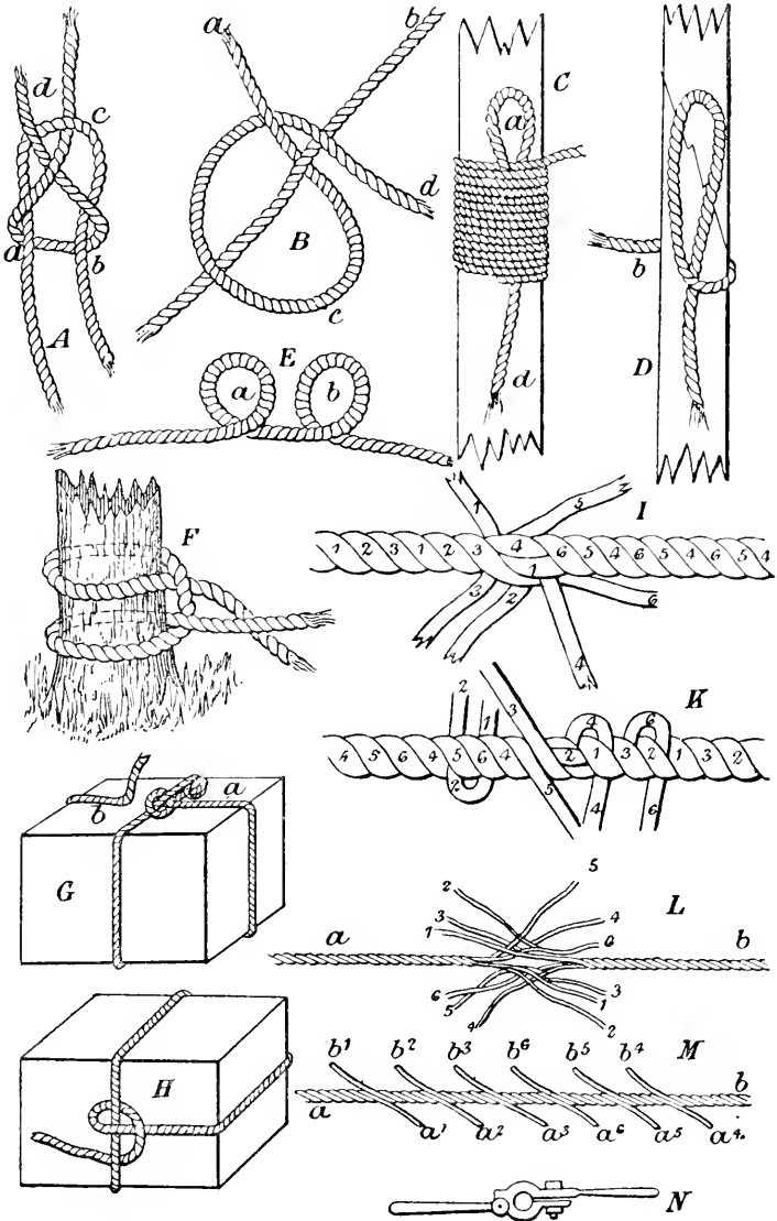
Knots and splices.
