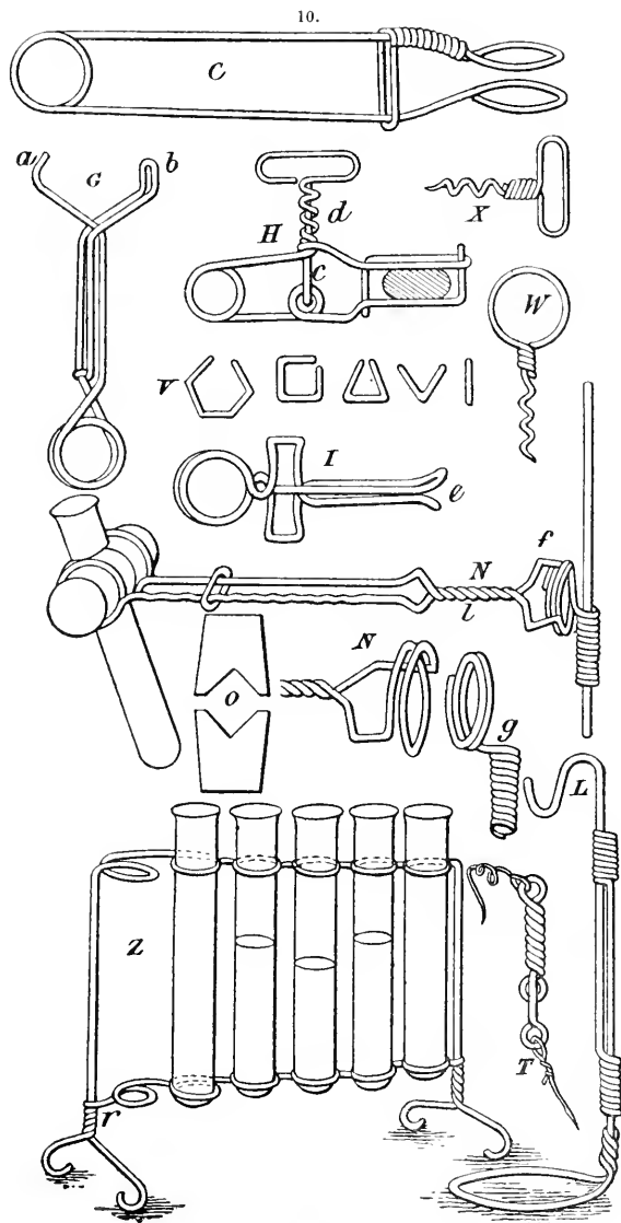
Wire apparatus for laboratory use.
