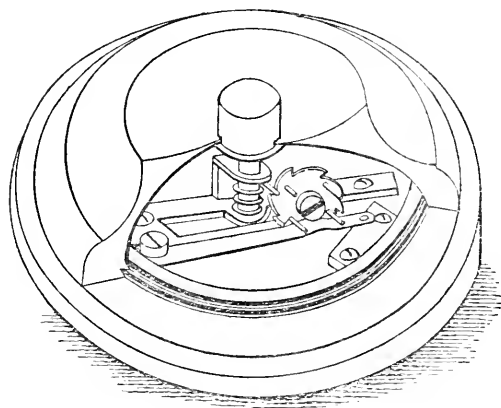
Salomon's commutator.
