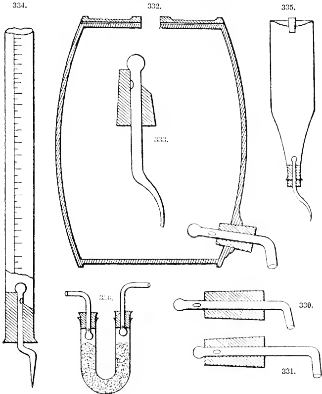
Simple forms of taps.
