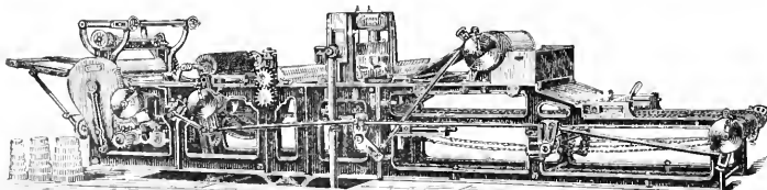
Latest Improved Patent Biscuit Cutting Machines.
