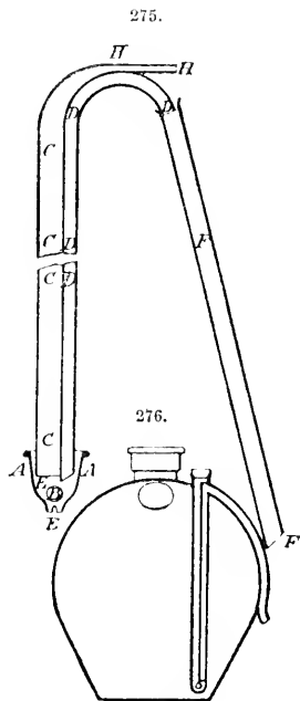
Siphon primed by blowing.
