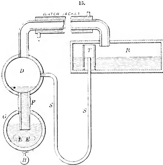
Perkins's cooling apparatus.
