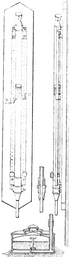
Glycerine barometer.
