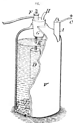
Latande-Chaperon battery.
