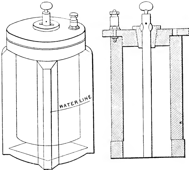
Holtzer battery.
