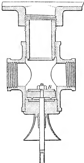
Victor valve, open.
