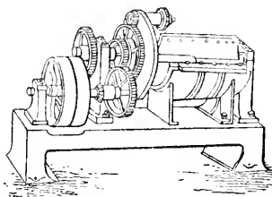
Machine for boring inside of curved plates.
