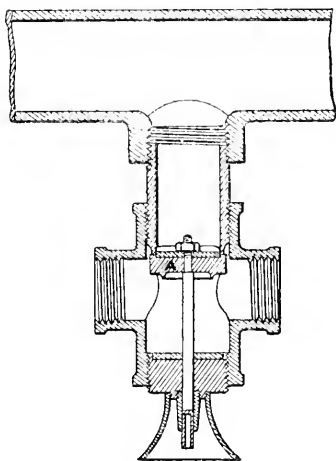
Victor valve, closed.
