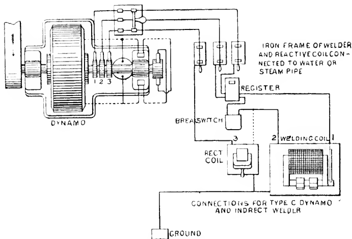
Electric welding apparatus.
