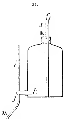
Mercury still.
