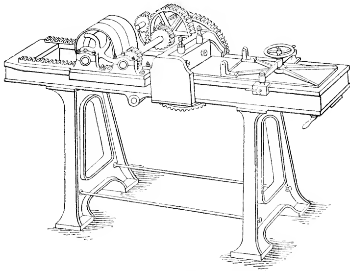
Draw bench for scraping back of plates.
