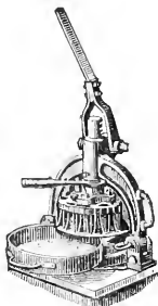
Patent Table Dough Divider.
