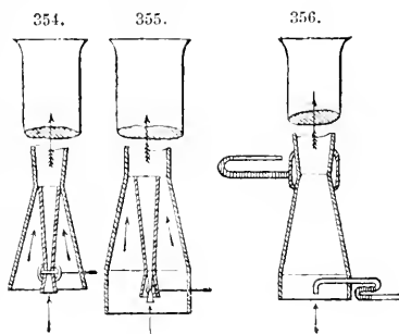
Multiplying anemometer.
