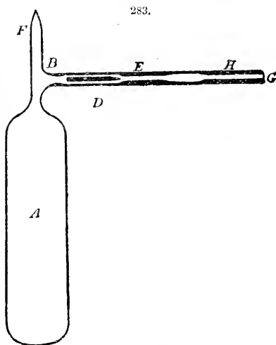
Sealing glass tubes.
