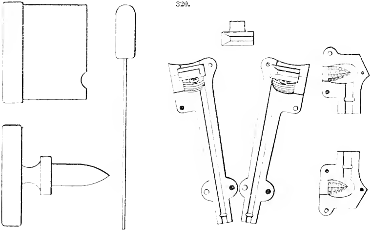
Pipe-moulders' tools.
