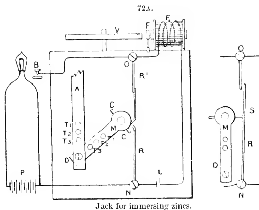
Jack for immersing zincs.
