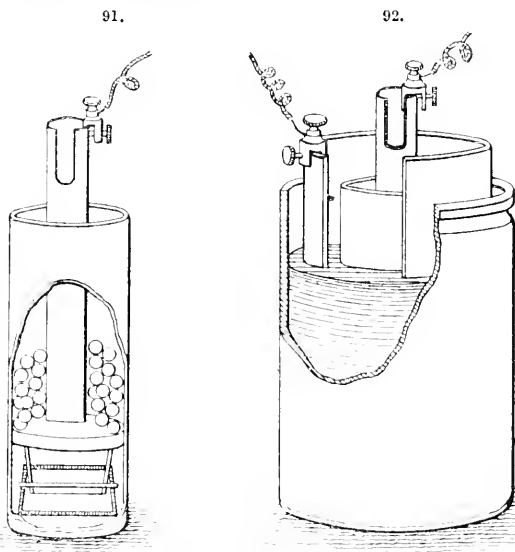
Radiguet's amalgamating supports.
