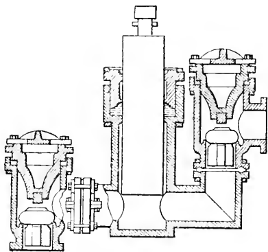
Stoneware acid pump.
