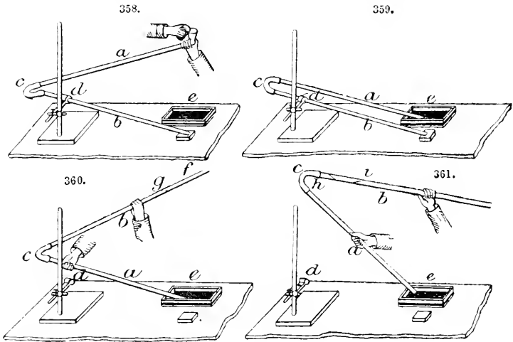
Exhausting barometer tubes.
