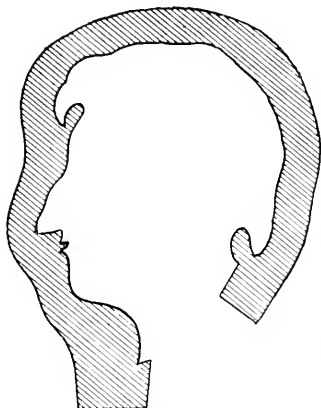
Simple close waste mould.
