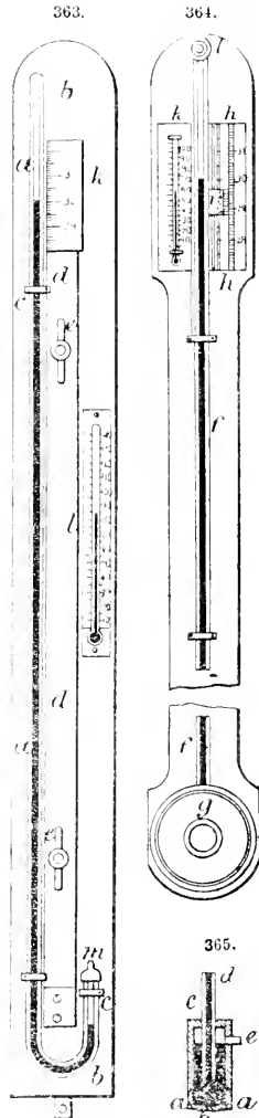
Siphon and cistern barometers.
