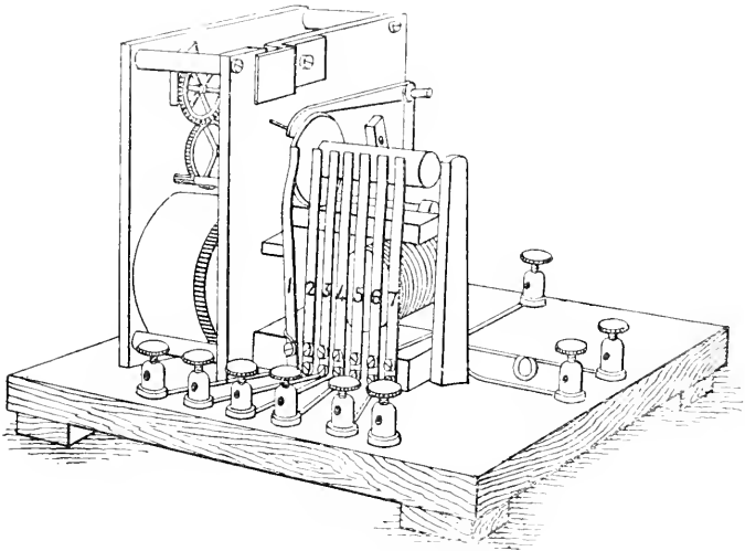
Automatic commutator.
