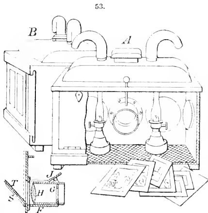
Reflecting lantern.
