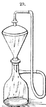
Filtering funnel.
