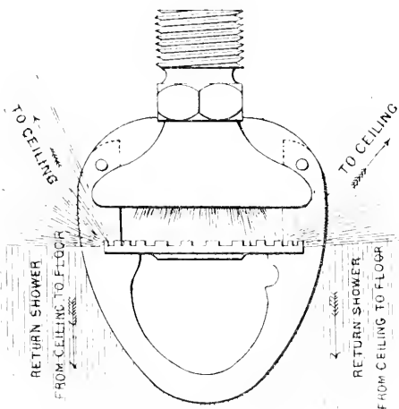
Grinnell sprinkler, open.
