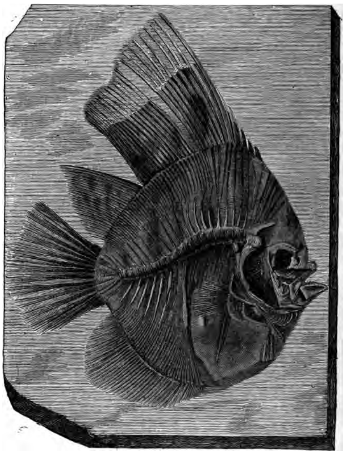
FOSSIL FISH.
