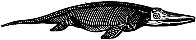
ICHTHYOSAURUS, OR FISH LIZARD.
