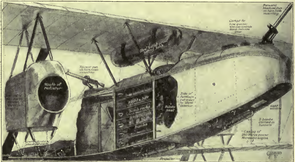
SECTIONAL DIAGRAM OF A GOTHA FIGHTING PLANE
