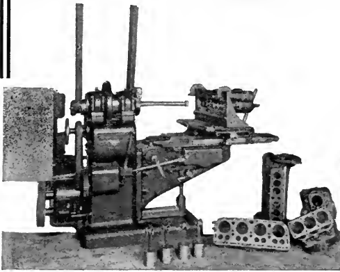
CYLINDER GRINDING
