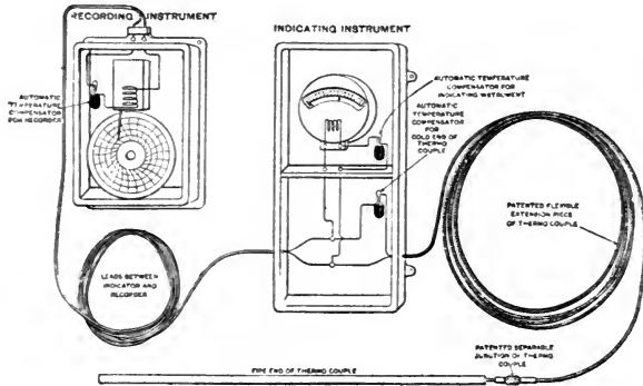
Fig. 10.—Bristol Recorder.
