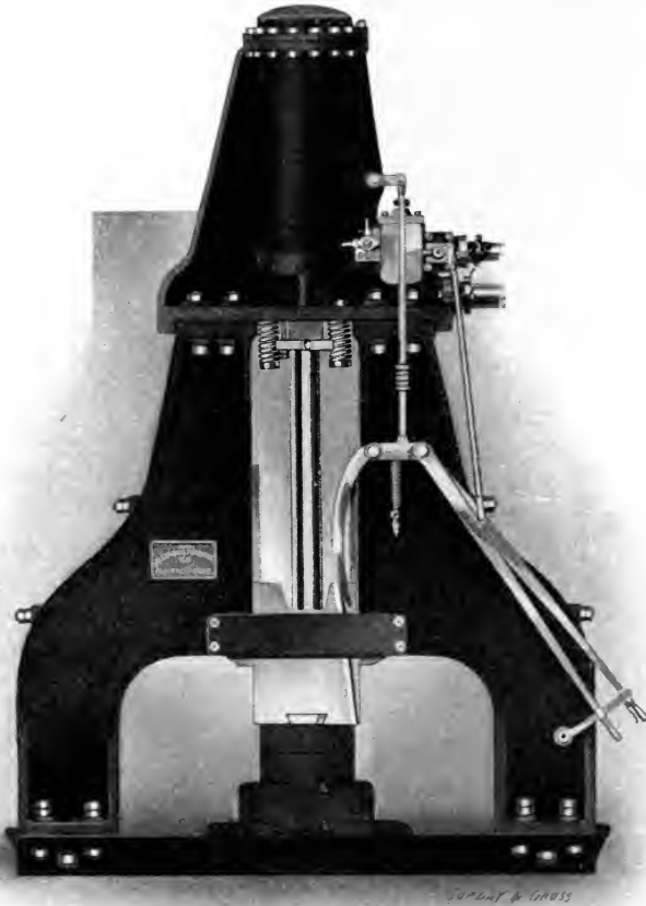
Fig. 75.—Double-Stand, Steam Hammer. (Alliance Machine Co.)
