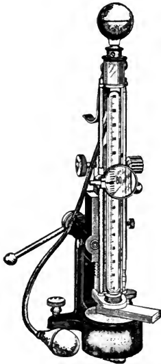
Fig. 3.—Shore Scleroscope.
