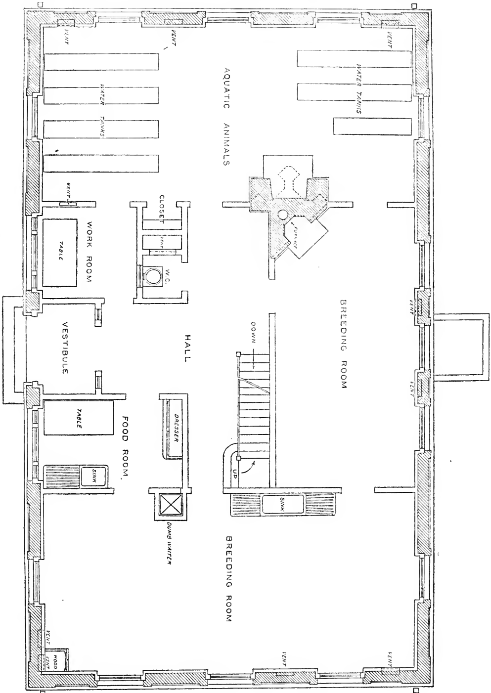
COLD SPRING HARBOR STATION, FIRST FLOOR PLAN.
