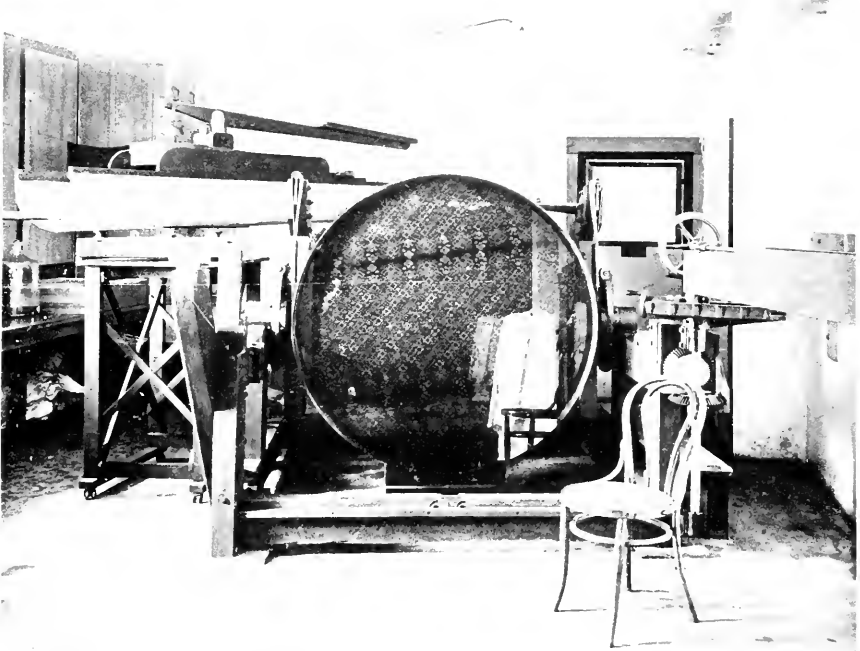
60-INCH MIRROR TURNED DOWN FOR TESTING.
