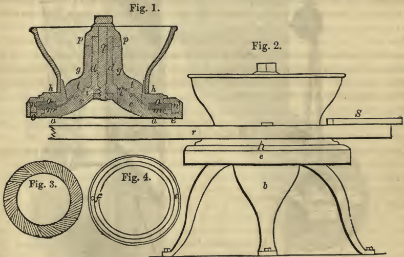
Fig. 1 is a vertical section of the mill; fig. 2 is an elevation; fig. 3 is a plan view of the movable rings; and fig. 4 is a plan view of the annular conductor. Similar letters refer to like parts.
