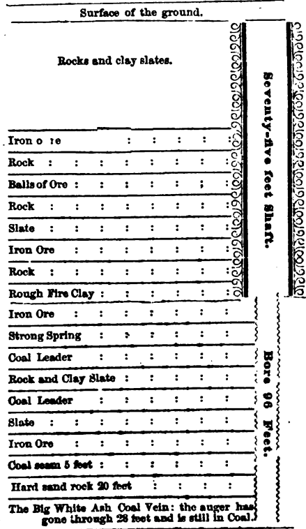
Diagram of M'Ginnis' Shaft, in the Town of Pottsville.
