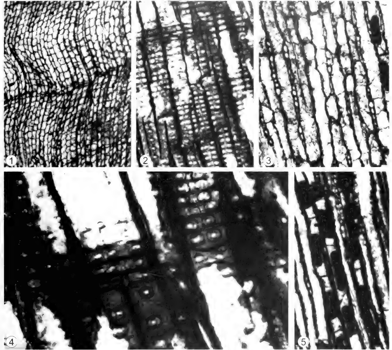
图版7-12 红杉型木 Sequoioxylon sequoianum (引自杜乃正, 1987)
