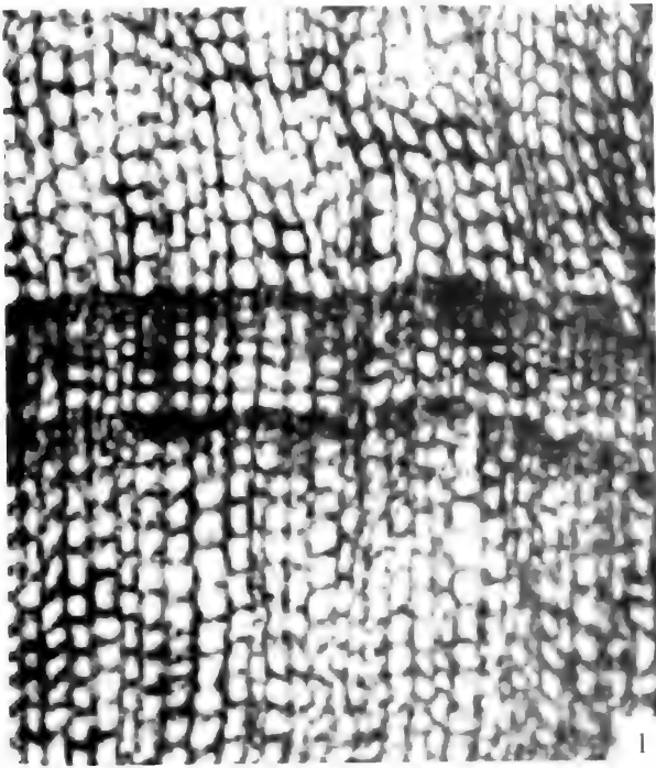
图版6-45 河北异木 Xenoxylon hopeiense Chang
