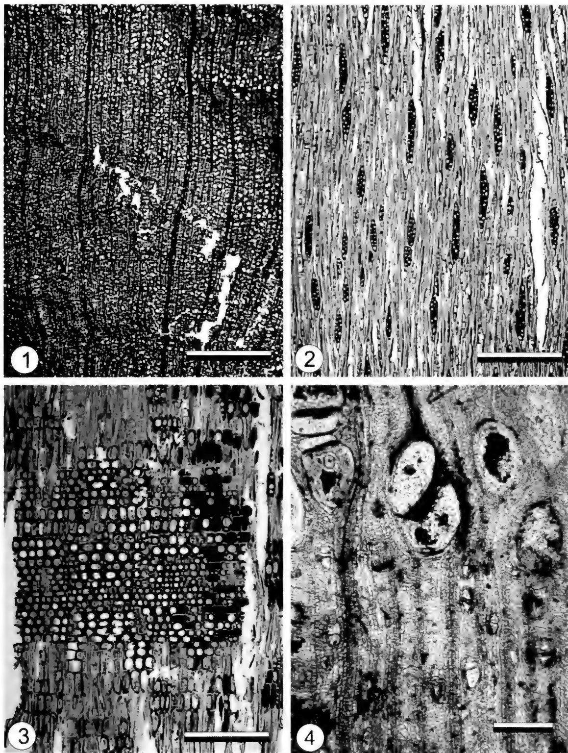
图版7-47 越桔型木 Vacciniaceoxylon vacciniumoides 等
