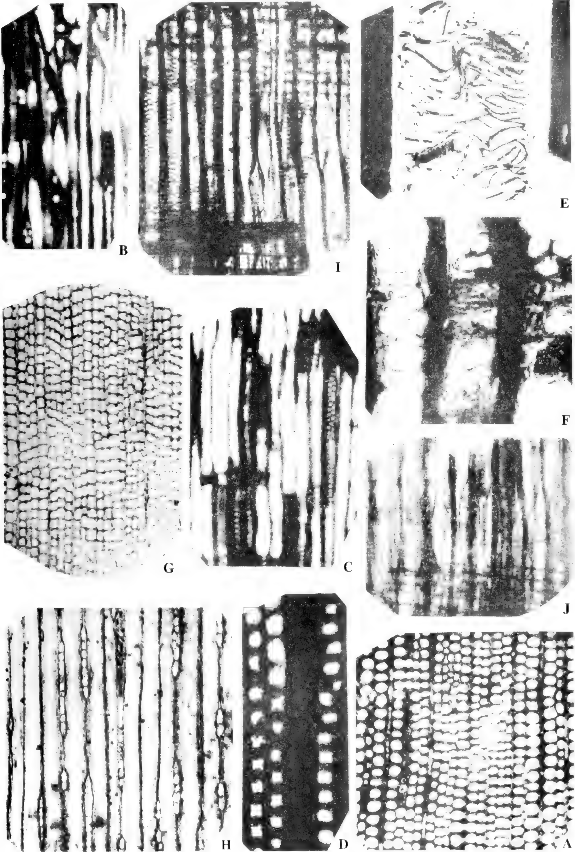
图版3-12 萨尼科达木 Cordiaoxylon sahnii (Hsü & Bose) Wang 等
