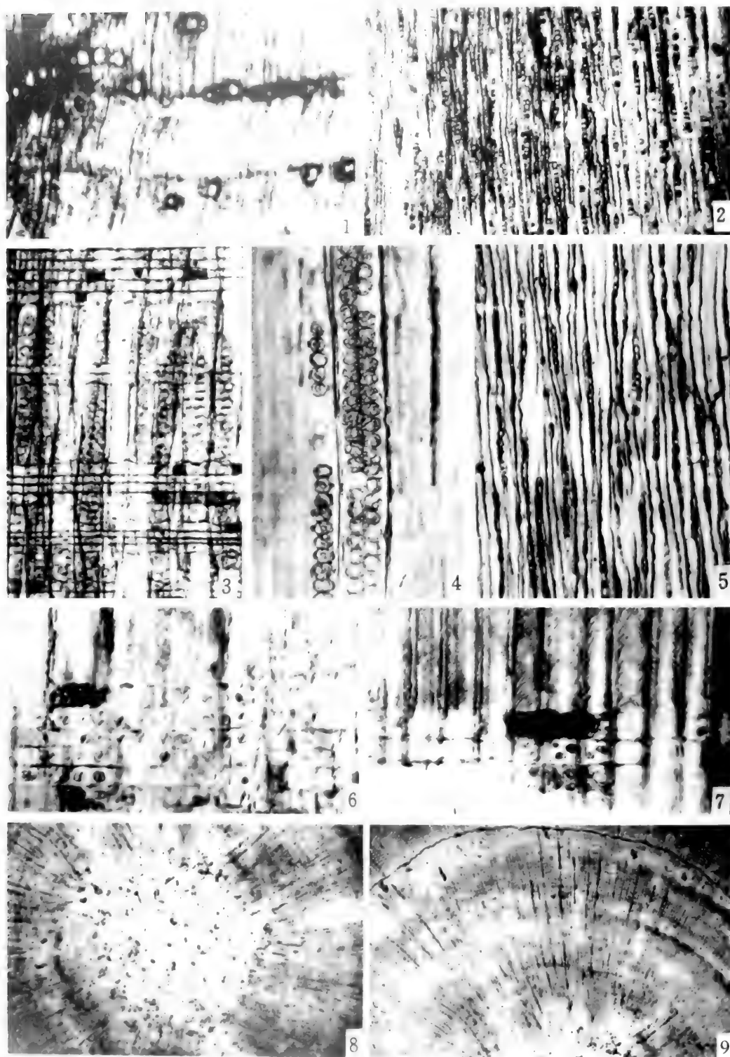
木 Protopiceoxylon chaoyangense Duan (图1-3)
