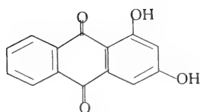
Purpuroxanthin
