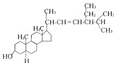
\Delta^{22} Stigmasterolm. 158 \sim 159^\circ\text{C}
