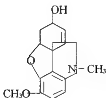
2-Epigalanthamine
