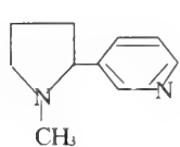
1-Nicotine
