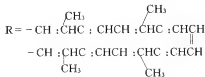
Xanthophyll C_{40}H_{50}O_2
