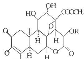
鸦胆子苦素A R = \text{COCH}_2\text{CH}(\text{CH}_3)_2 鸦胆子苦素B R = \text{COCH}_3 鸦胆子苦素C R = \text{COCH}=\text{C}(\text{CH}_3)-\text{C}(\text{OH})(\text{CH}_3)_2
