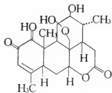
m. 238 ~ 242 ^{\circ}\text{C} Chaparrinone
