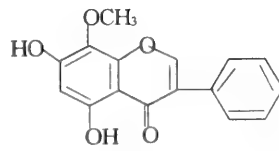
Wogonin
