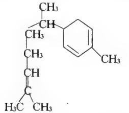
b. (-): 134 ^{\circ} C (14mmHg) Zingiberene
