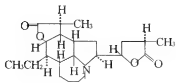
TuberoSTEMONINE
