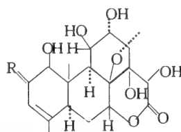
鸦胆子苦素D R = O 鸦胆子苦素E R = \alpha\text{-OH}, \beta\text{-H}
