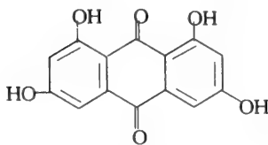
Emodin
