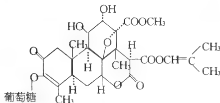
鸦胆子甙B
