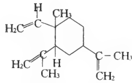
\beta -Elemene
