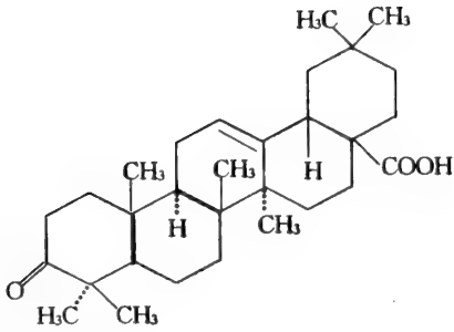
Oleanonic acid
