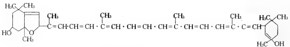
Chrysanthemaxanthin
