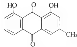
Chrysophanic acid
