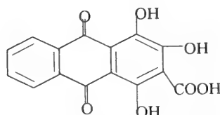
Pseudopurpurin
