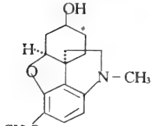
m. (-): 120~121°C (±): 98~99°C Lycoramine
