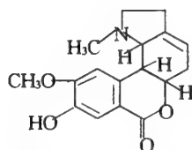
9-Demethylhomolycorine
