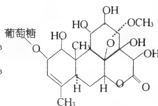
鸦胆子甙
