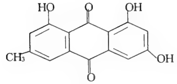
Emodin
