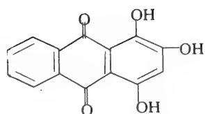
Purpurin
