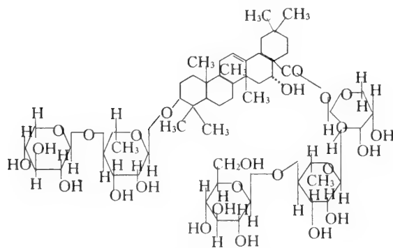
Helianthoside B
