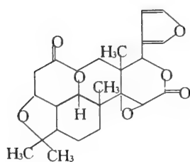
Obaculactone
