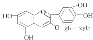
Cyanidin-3-xylosyl-glucoside
