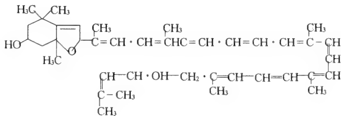
Flavoxanthin
