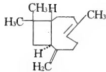
Caryophyllene
