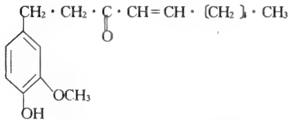
b. 201 ~ 203 ^{\circ} C (2 ~ 2.5mmHg) Shogaol
