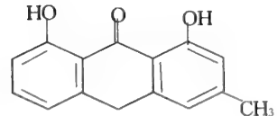
Chrysophanic acid anthrone
