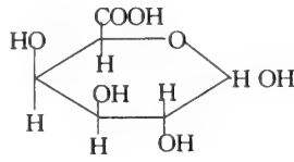
D-Galacturonic acid
