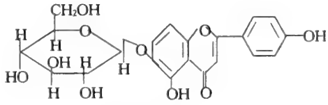
Homoplantaginin
