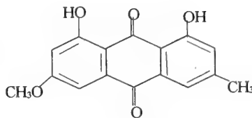
Physcion
