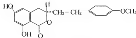
Agrimonolide
