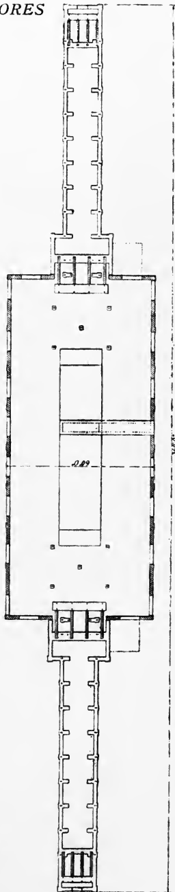
FIG. 4.—HEGELER ROASTING FURNACE. PLAN OF FURNACE AND STIRRING MECHANISM.
