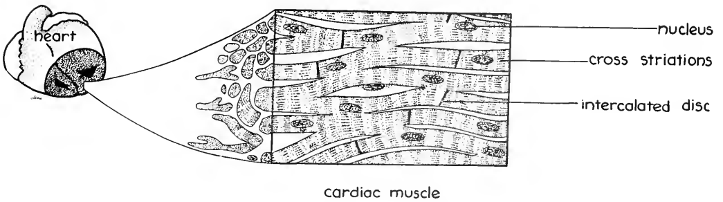
Fig. 4-5. Types of contractile tissue.
