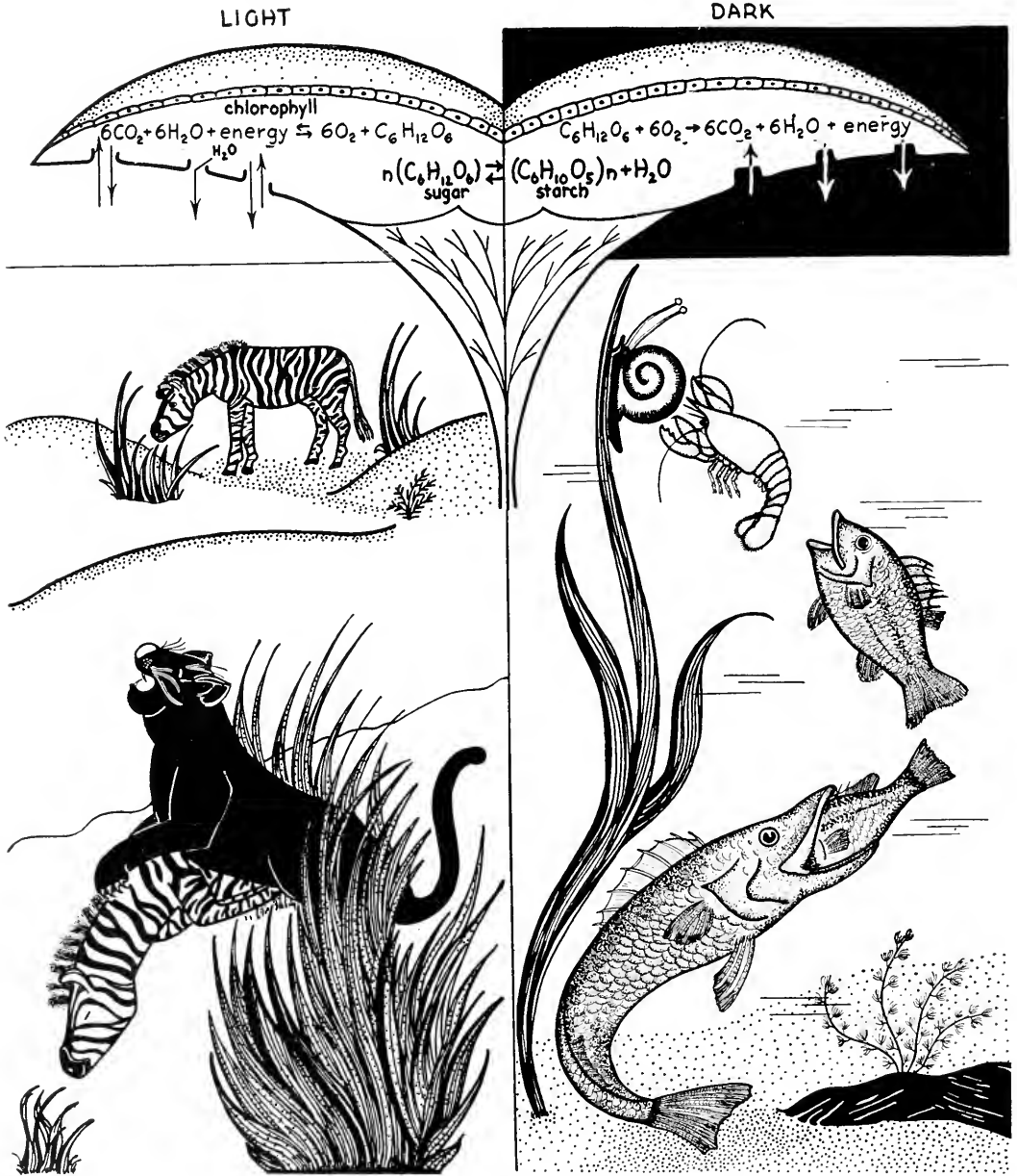
Fig. 5-7. Food chains. In each case the chain starts with the plant where photosynthesis produces the first food; the plants are eaten by herbivores, which are in turn eaten by a series of carnivores, in one case ending with the large fish and the other with the leopard.
