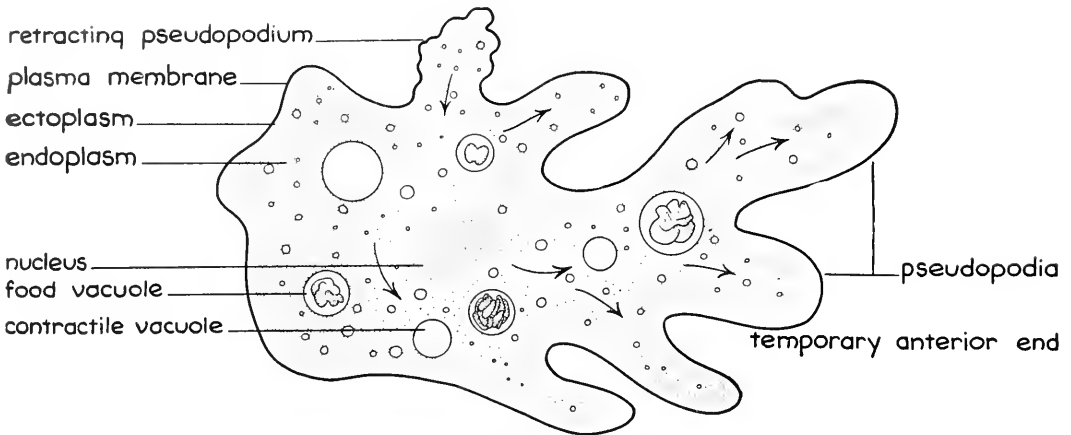
Fig. 7-3. Amoeba with internal anatomy shown in detail.
