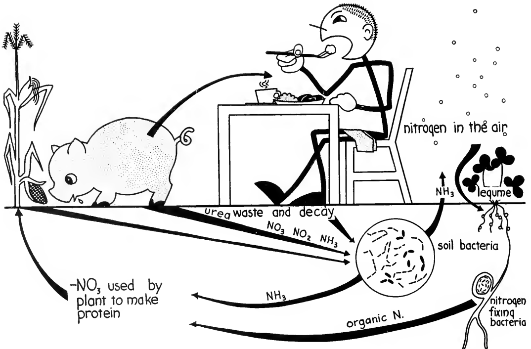
Fig. 5-5. The nitrogen cycle.
