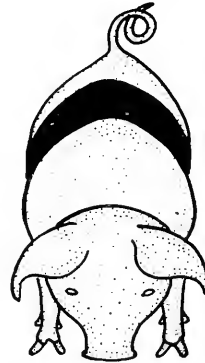
Fig. 4-8. Orientation of an animal possessing bilateral symmetry.
