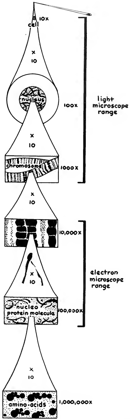
Fig. 2-17. Relative sizes of things that are of interest to the biologist. Magnifications greater than 100,000 are useful to the physicist and chemist.
