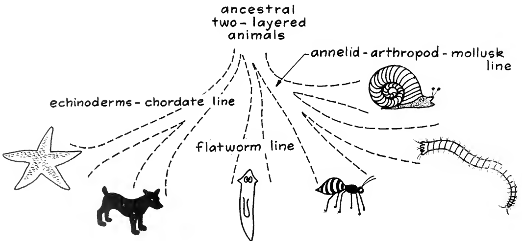
Fig. 13-5. The coelenterates probably gave rise to the echinoderm-chordate line, the flatworm line, and the annelid-arthropod-mollusk line.
