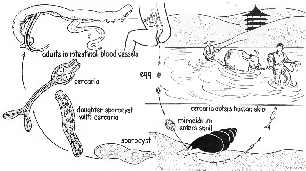
Fig. 9-10. Life history of a typical human blood fluke.
