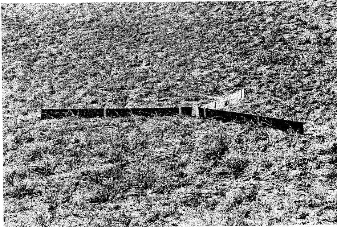
Figure 4: Drift fence array showing radiating fins around a central pitfall can, with an additional pitfall can at the end of each fin.
