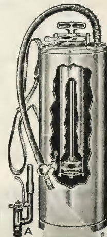
PATENTED. The Auto Spray Pump.
