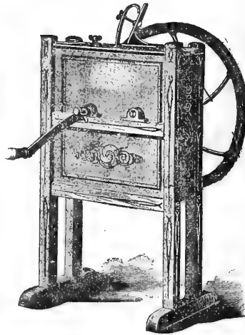
No. 5. ONE HOLE. Capacity, 125 bushels per day; single spout; left hand. Corn and cobs separated. $6.00.
