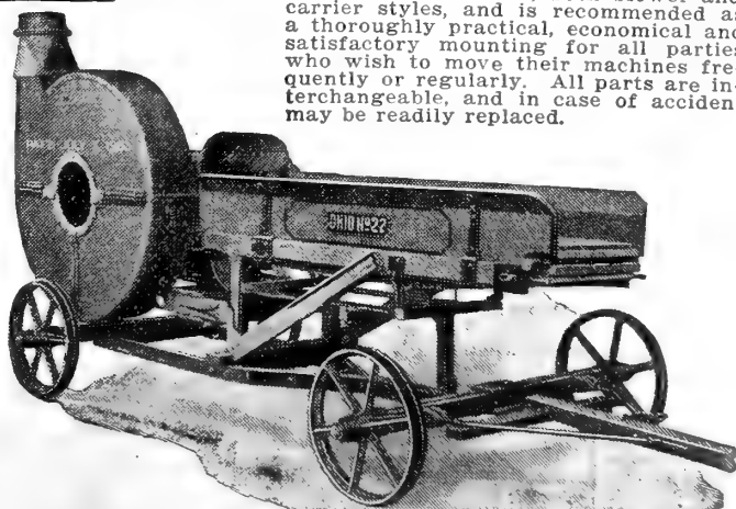
Price of Truck, without neck yoke or double trees, weight 600 lbs., $50.00. Less 30 per cent. Retail.
