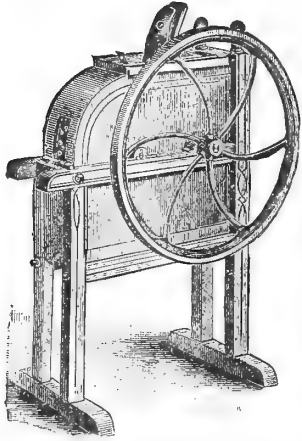
No. 3. ONE HOLE. Separates corn and cob. Fan will clean corn for market. Corn discharged beneath Sheller, cobs at end. Easily adjusted for large or small ears. Capacity, 125 bus. a day. Plain, $6.50. With fan, $7.00.
