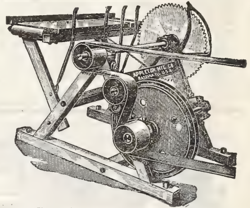
New Style Tilting Table Pole Saw.
