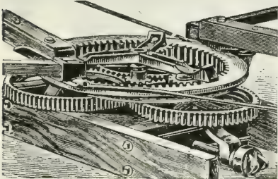
Two Horse-power, Geared.
