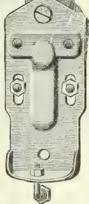
Bracket for Track Joints.
