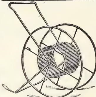
No. 10 All-Steel Reel. Diameter of wheels... 22 in. Diameter of drum.... 9 in. Width between wheel... 10 in. Length of handle.... 28 in. Capacity, 100 ft 3/4-in. hose. Weight about 17 lbs. The large wheels roll easily over rough or soft ground. Nothing to get out of order. Rigid—Durable—Attractive. Price .....
