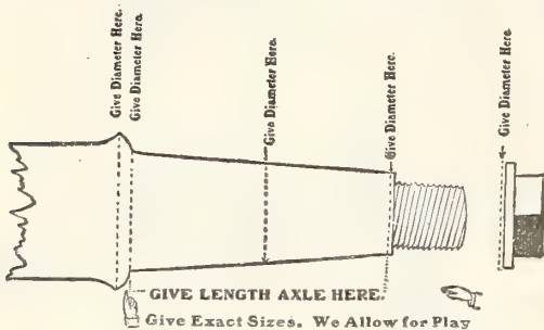
DIAGRAM SHOWING HOW TO MEASURE YOUR SKEINS
