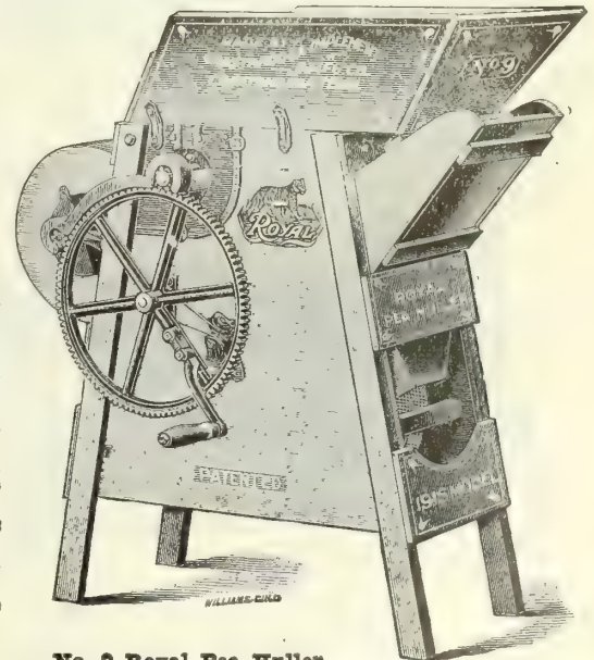
No. 9 Royal Pea Huller.
