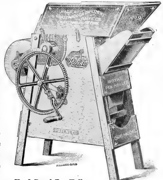
No. 9 Royal Pea Huller.
