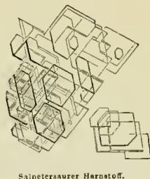
Salpetersaurer Harnstoff.
