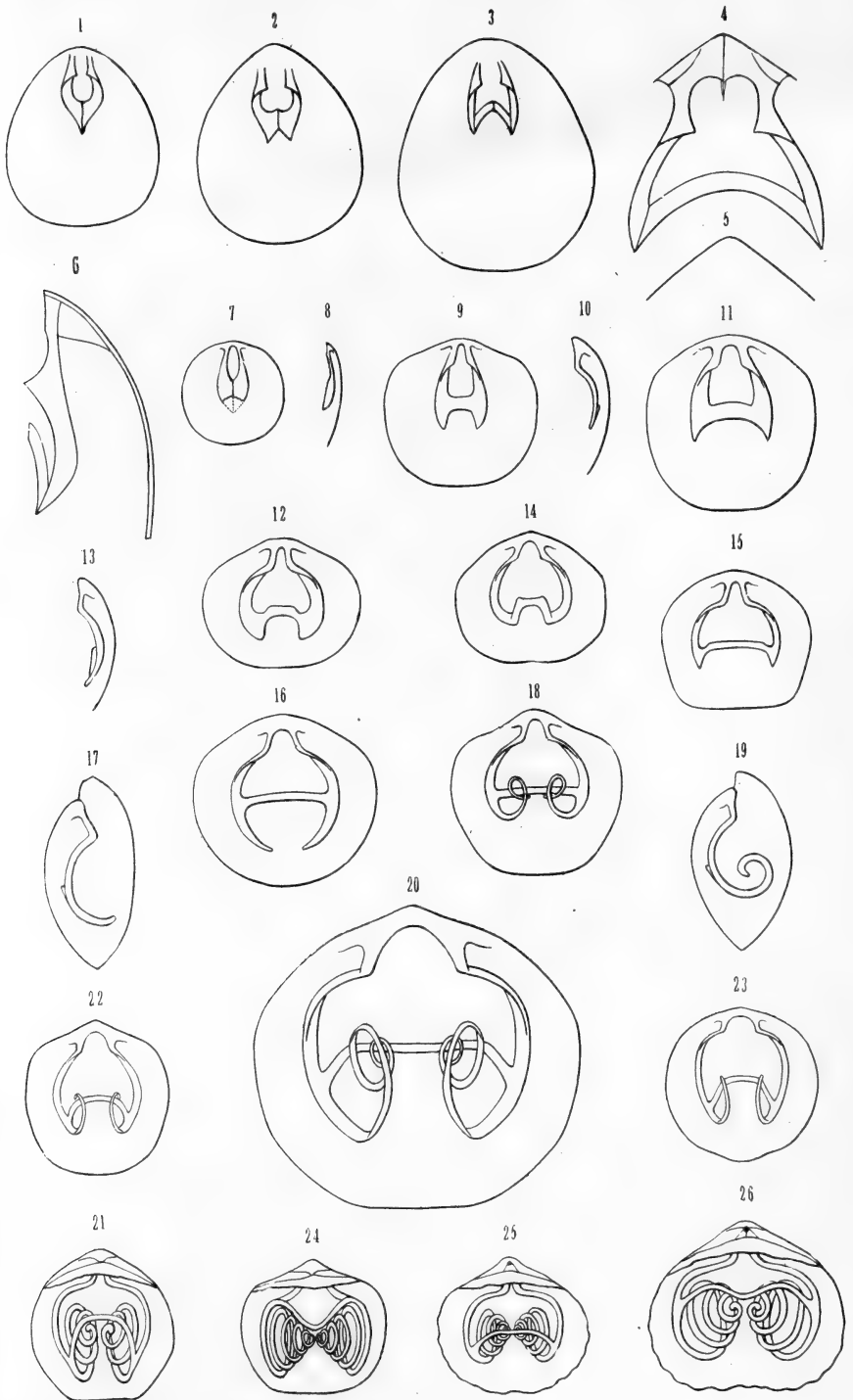
BRACHIAL SUPPORTS IN DIELASMA AND ZYGOSPIRA .
