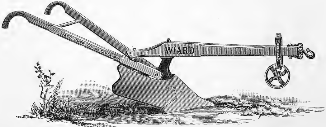
ONE HORSE SWIVEL PLOW. Price, $8.00.
