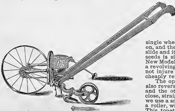
IRON AGE COMBINED SEED DRILL AND WHEEL HOE.
