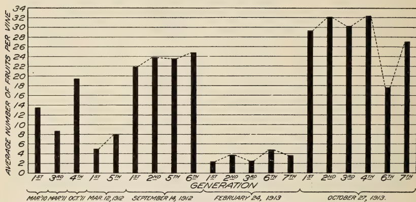
FIG. 7.—Average yields of Royal Red tomato generations, the number of fruits being indicated by heavy lines and simultaneous plantings connected by dotted lines.
