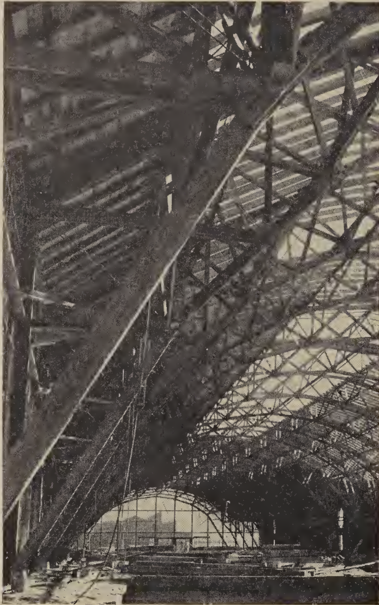
Two hundred-foot trussed timber arches in building for 1939 Golden Gate International Exposition, San Francisco.
