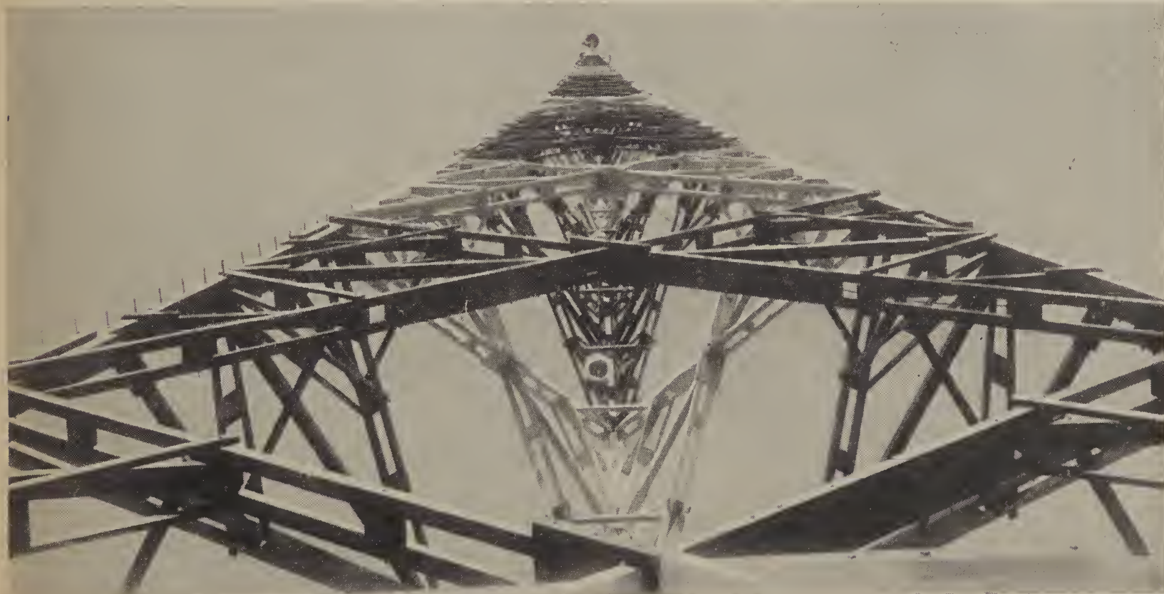
Below: Mole's-eye view of radio station WRVA tower, Richmond, Va., built of timber with modern connectors.
