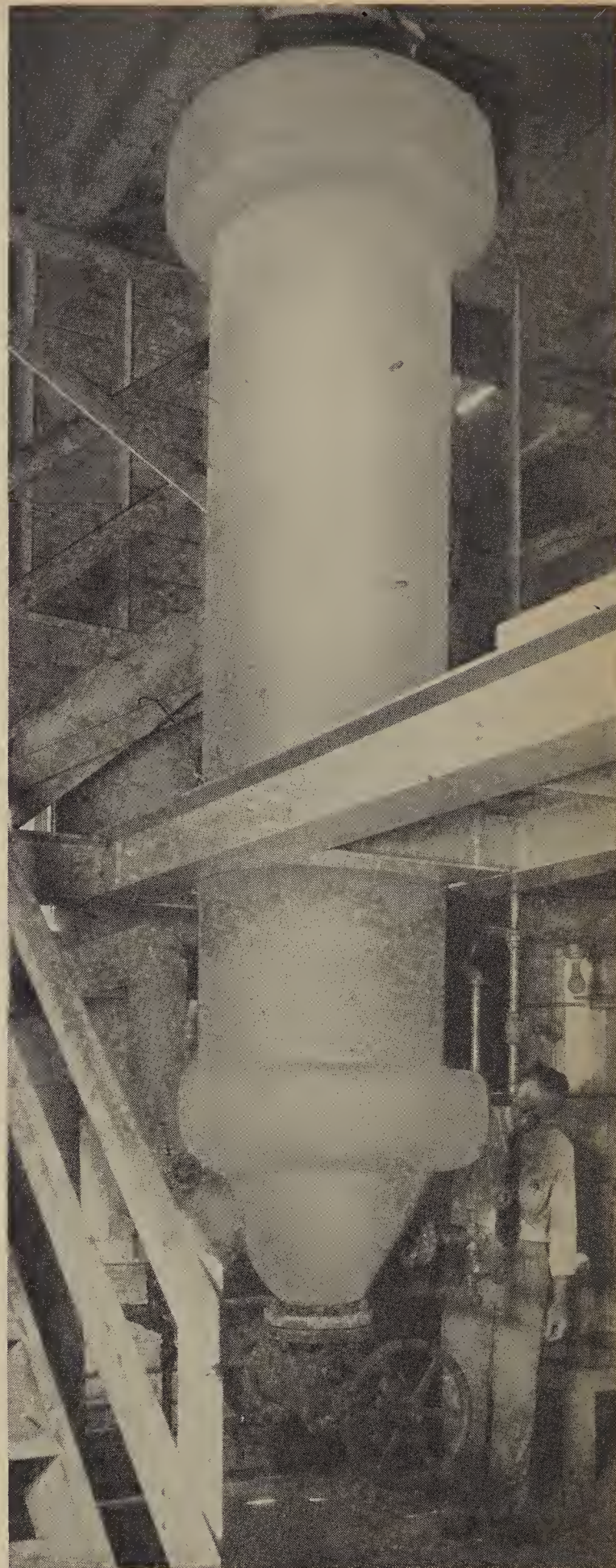
Percolator for production of grain alcohol from wood.
