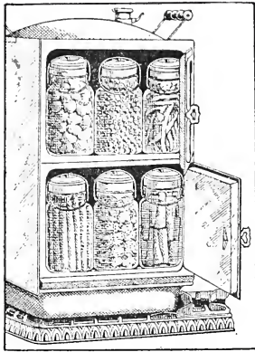
FIG. 7. Home canner and steam cooker holding 14 quart jars. Requires same time as hot-water bath.
