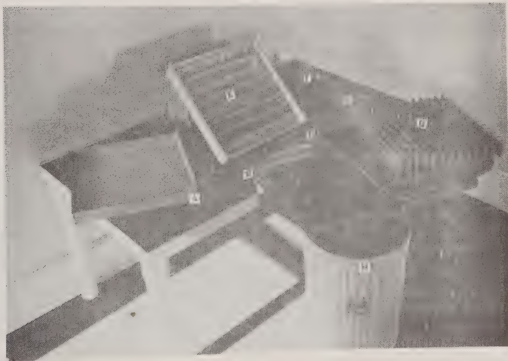
Figure 3.--Equipment set up for extracting cocoons from cocoon-formation flats. A, Empty flat from which cross section has been removed; B, wooden hopper; C, sieve in position on hopper; D, cross section in position for extracting cocoon-laden soil; E, tray for cocoon-storage vials in position to receive cocoons; F, alcohol lamp; G, forceps; H, ash can into which fits hopper B.
