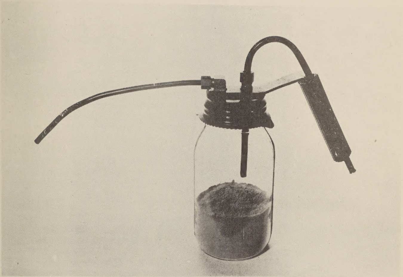
Figure 2.—Dust gun, showing tube compression couplings, gaskets, U-shaped air-intake tube, dust supply, discharge tube, and parts forming the grip.
