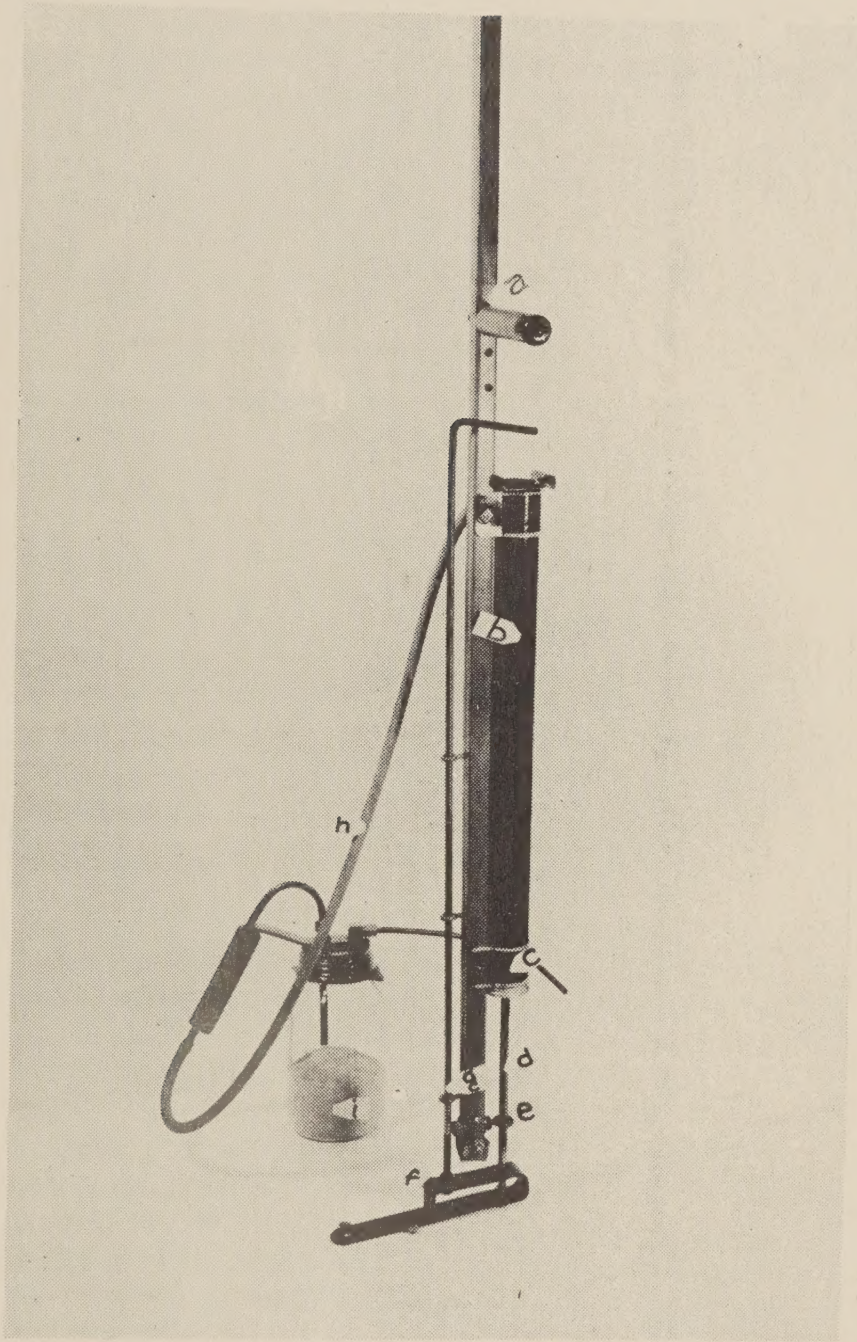
Figure 3.—Details of the air pump: (a) Adjustable staff handle, (b) medium-sized tire pump, (c) sheet-metal clamp, (d) pump plunger rod, (e) plunger-rod eyebolt, (f) foot brace, (g) guide rod, (h) air hose, and (i) dust gun. A simpler foot brace may be made of wood, as described on page 1.
