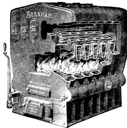
The Burnham Boiler. Interior View.
