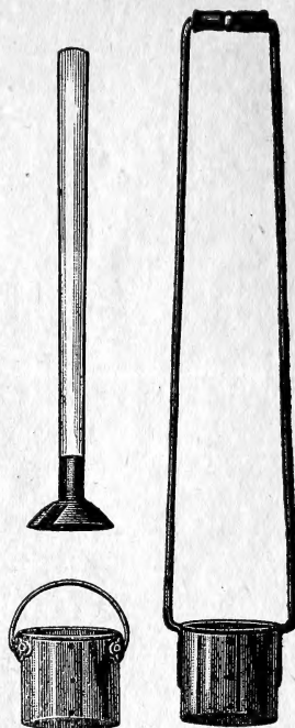
TRANSPANTER. EXCAVATOR.
