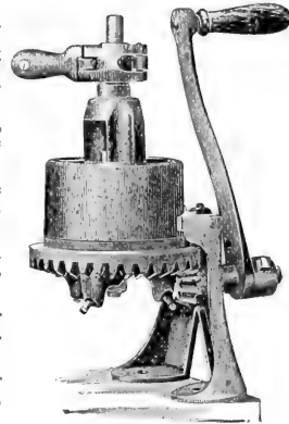
No. 1 CRANK.
