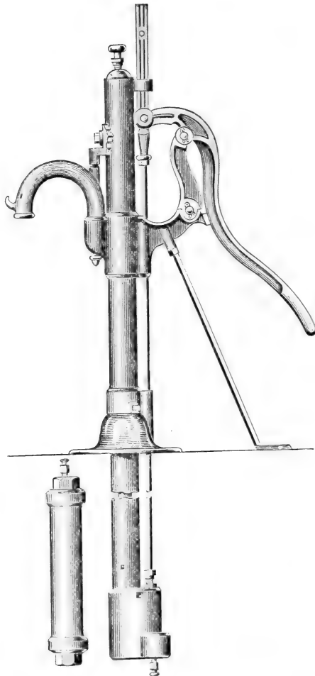
The Thomas Double-Acting Force and Lift Pump.
