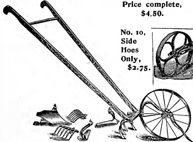
No. 1 "IRON AGE" Combined Harrow and Cultivator
