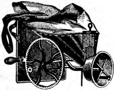
Cahoon Hand Seeder. Price $4.00.
