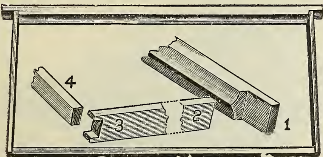
THICK-TOP FRAME.
