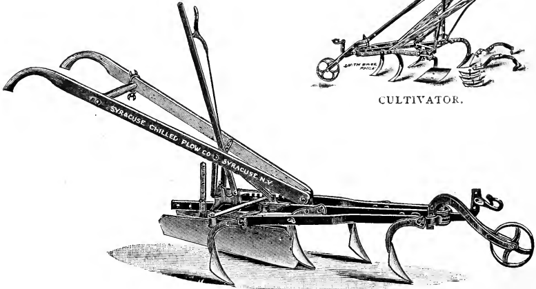
SYRACUSE CULTIVATOR.
