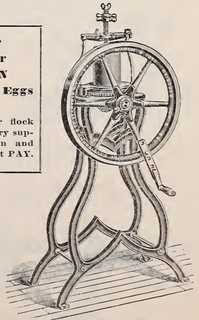
WEBSTER & HANNUM GREEN BONE MILL No. 6.
