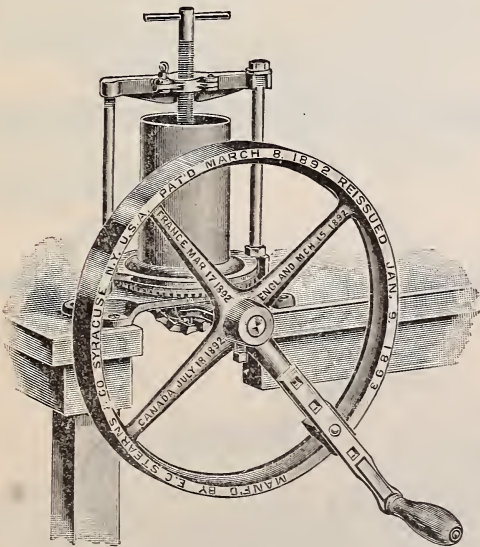
WEBSTER & HANNUM GREEN BONE MILL NO. 4.
