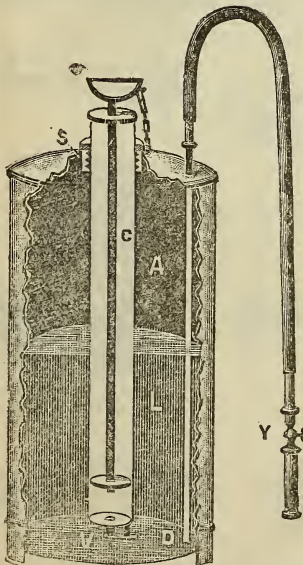
PHILIPPS COMPRESSED AIR SPRAYER
