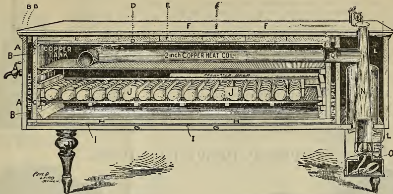
SECTIONAL VIEW OF NEW NO. 3 HOT WATER INCUBATOR.
