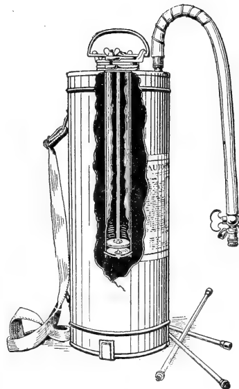
AUTO-SPRAY SHOWING WORKING PARTS.
