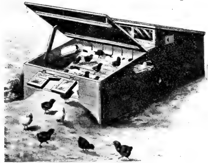
STYLE A, FRONT VIEW.
