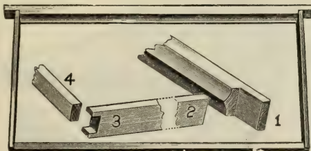
THICK-TOP FRAME.
