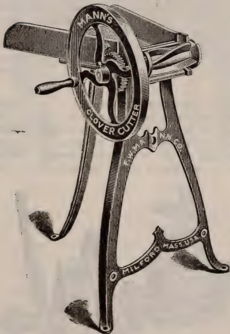
Mann's Clover Cutter Mounted.
