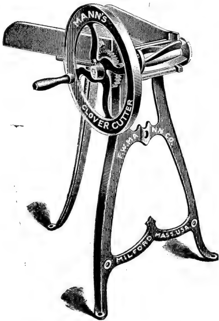
Mann's Clover Cutter Mounted.
