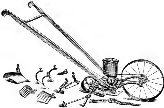
No. 15. Combined Single Wheel Hoe, Hill and Drill Seeder.
