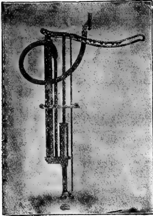
THE SPRAMOTOR, JR.
