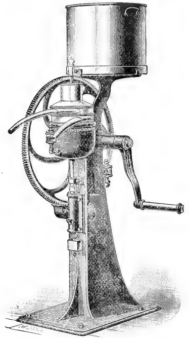
HIGH-FRAME "BABY" No. 3. Actual Capacity, 1,000 Lbs. per Hour. Price, $200.00.
