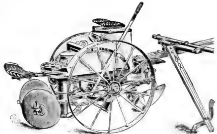
THE "NEW MODEL" SEED DRILL.
