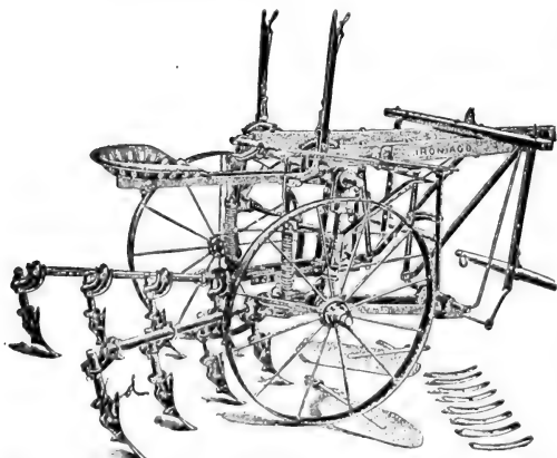
No. 80 "Iron Age" Pivot Wheel Riding Cultivator.
