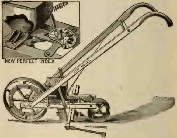
New Model Seed Drill, $7.50.
