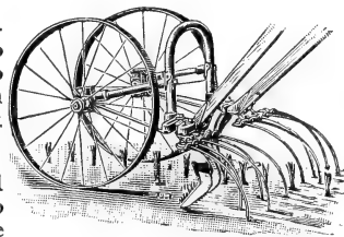
Fig. 81 Double Weeder Attachment Price per pair, $1.00
