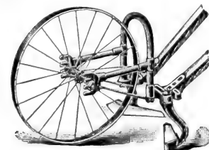
Showing the Double Wheel Hoe Set up as a Single Wheel.
